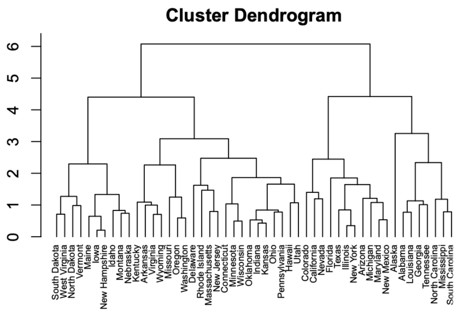
Figura 1.14: US Arrest Hierarchical Clustering, retomado de Chang (2020, p 216) [Cha20]
