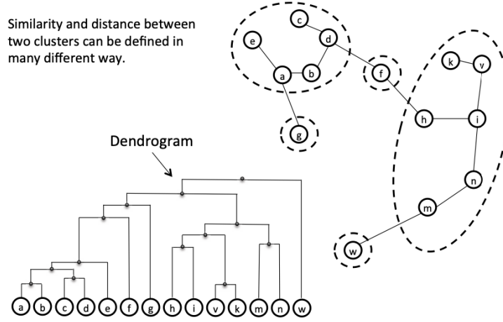
Figura 1.15: Agglomerative Clustering Algorithm and Dendrogram, retomado de Chang (2020, p 219) [Cha20]
